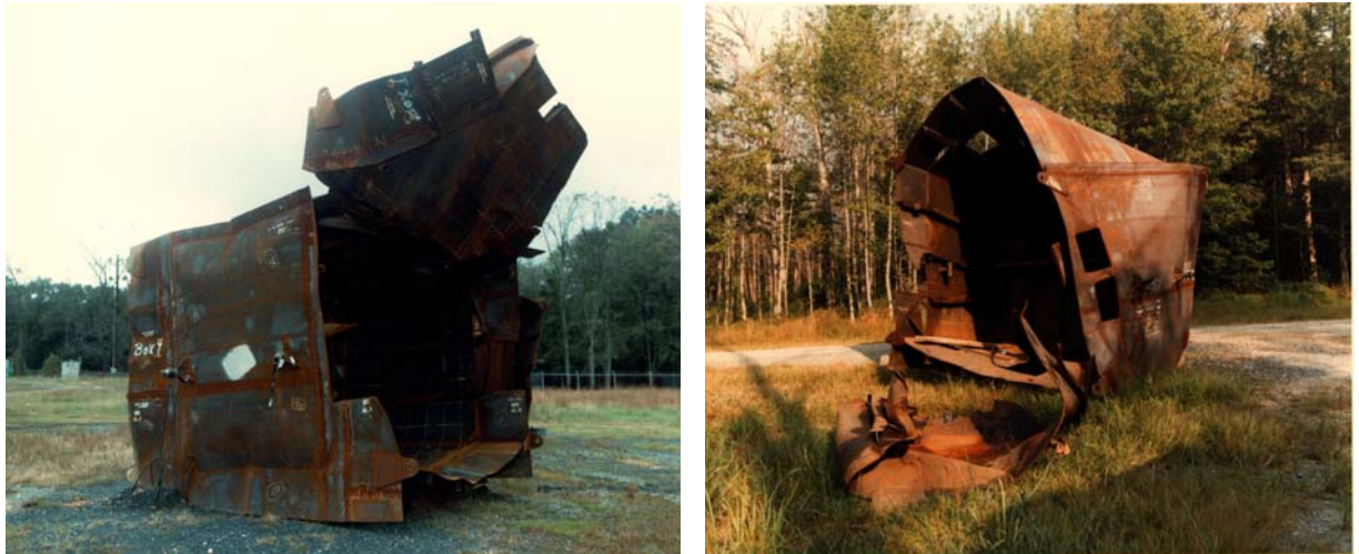
Structural failure from HE detonation Structural failure from propellant burn
