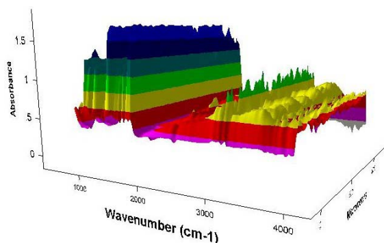
Fig 4: Nitramine FTIR imaging along the LOVA grain
