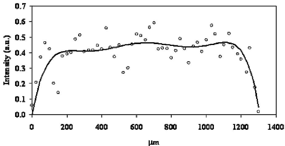
Fig 5: Nitramine FTIR distribution across the web size grain
