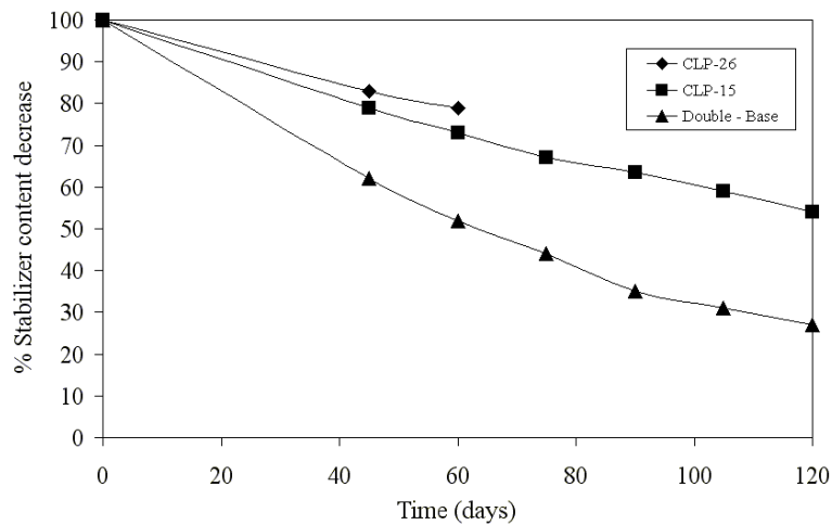
Fig. 2 – Accelerated ageing - Stabilizer depletion of Nitramine compared to DB propellants.
