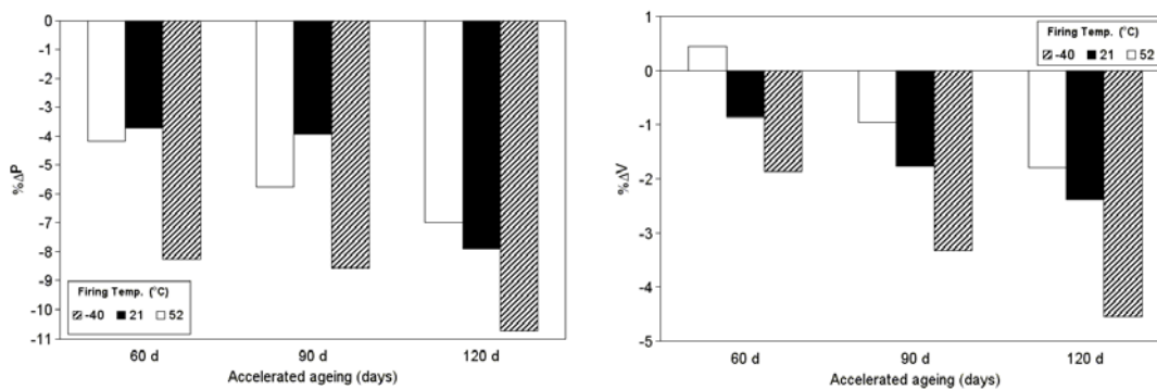
Fig 6 – Ballistic Performances after accelerated ageing
