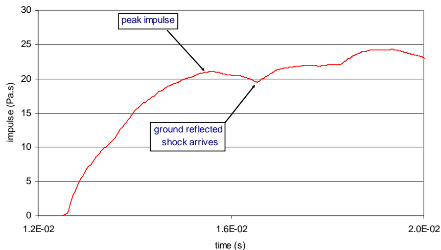
Figure 5 Positive impulse at upper gauge position, 6m from RX1100 charge with 2kg steel case
