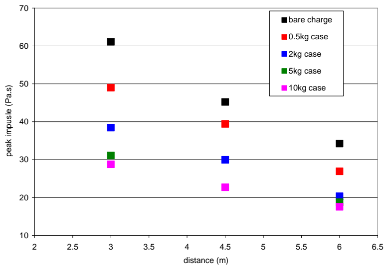
Figure 7 Peak impulses measured for RX1100 charges with steel cases
