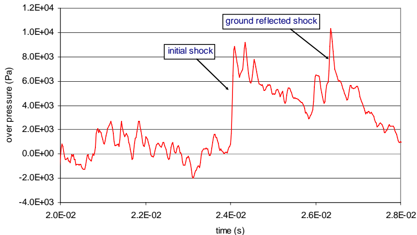
Figure 6 Pressure recorded at upper gauge position, 10m from RX1100 charge with 2kg steel case
