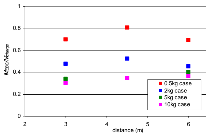
Figure 9 Case effects inferred from RX1100/steel case impulse results
