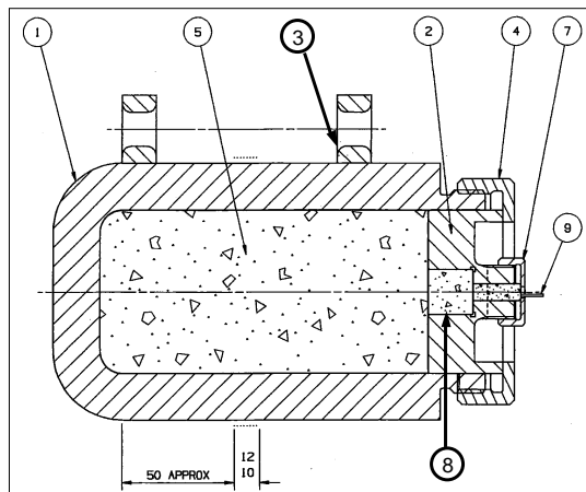
Typical Charge Configuration
