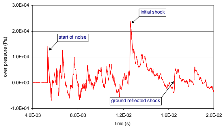
Figure 4 Pressure recorded at upper gauge position, 6m from RX1100 charge with 2kg steel case
