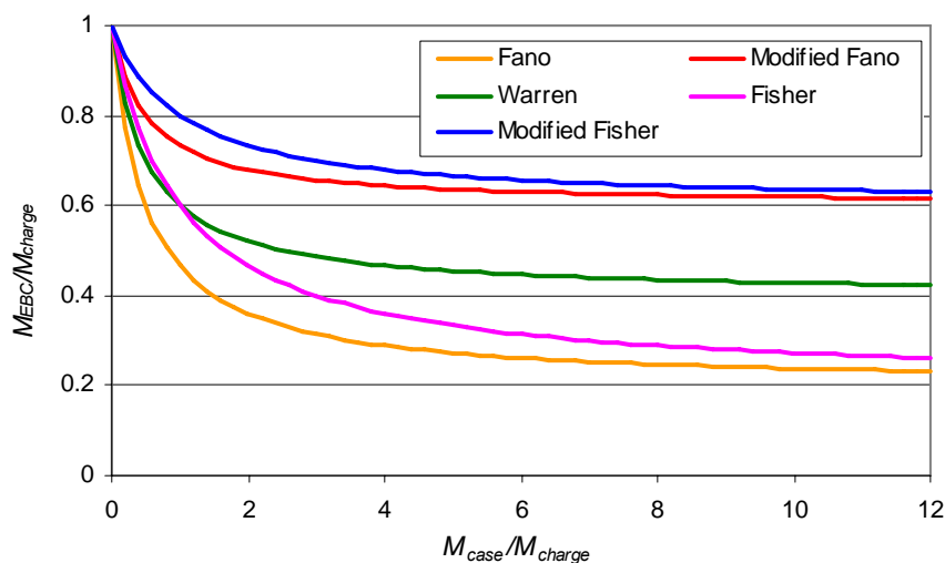
Figure 1 Effects computed using existing algorithms
