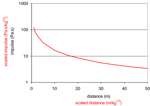
Figure 8 Peak impulses computed for 1kg spherical TNT charge
