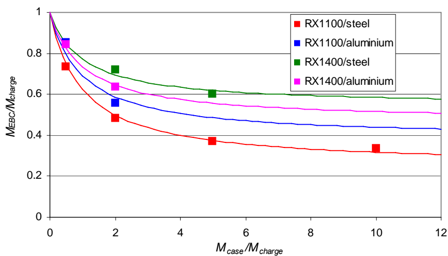
Figure 11 Case effects as a function of case mass for different charge/case systems together with fitted Fisher curves
