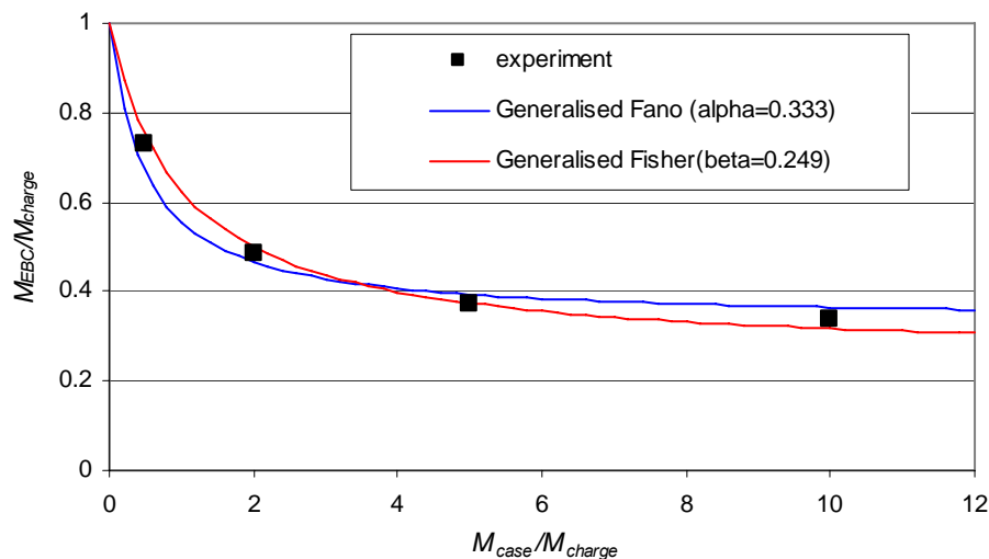
Figure 10 Case effects as a function of case mass for RX1100/steel case systems
