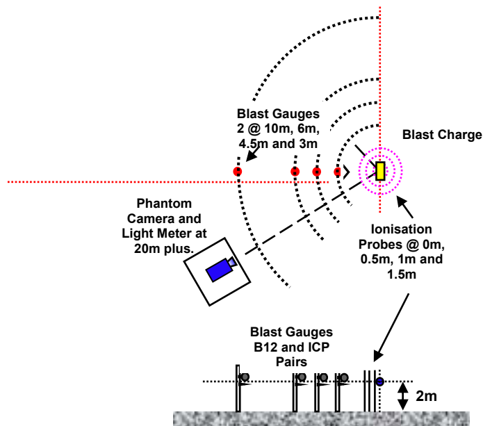
Figure 3 Layout of gauges (and other instrumentation)
