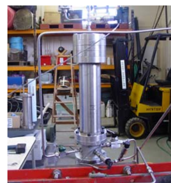
Figure 6: Gel expulsion test rig
